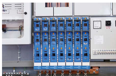
Effizienter Transformatorschutz Efficient protection for transformers
